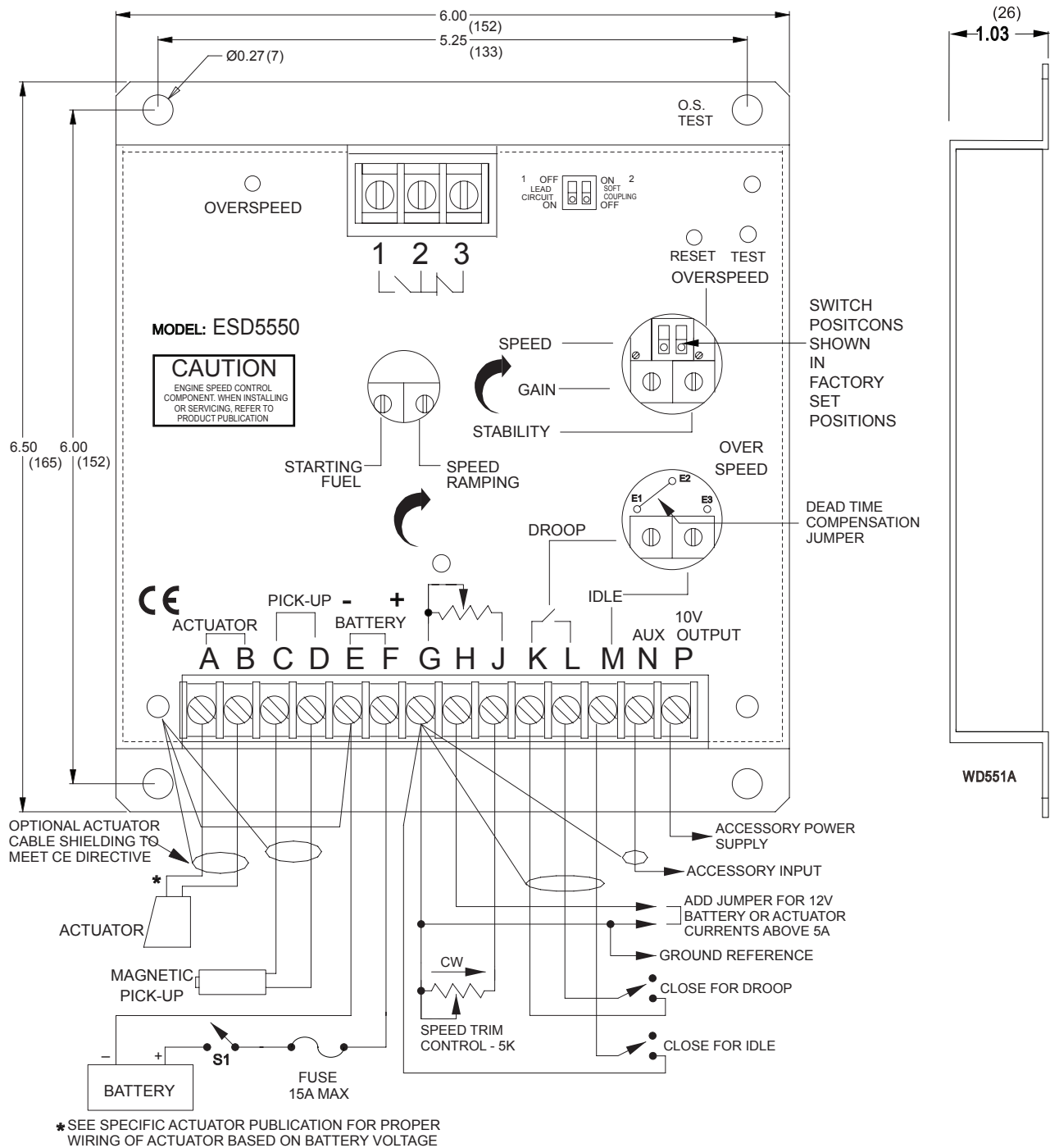
DIAGRAM 1. ESD550E Series Wiring Diagram and Outline
